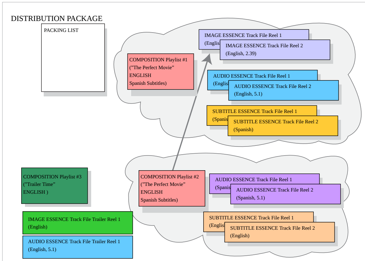
Figure 7: Example Distribution Package
