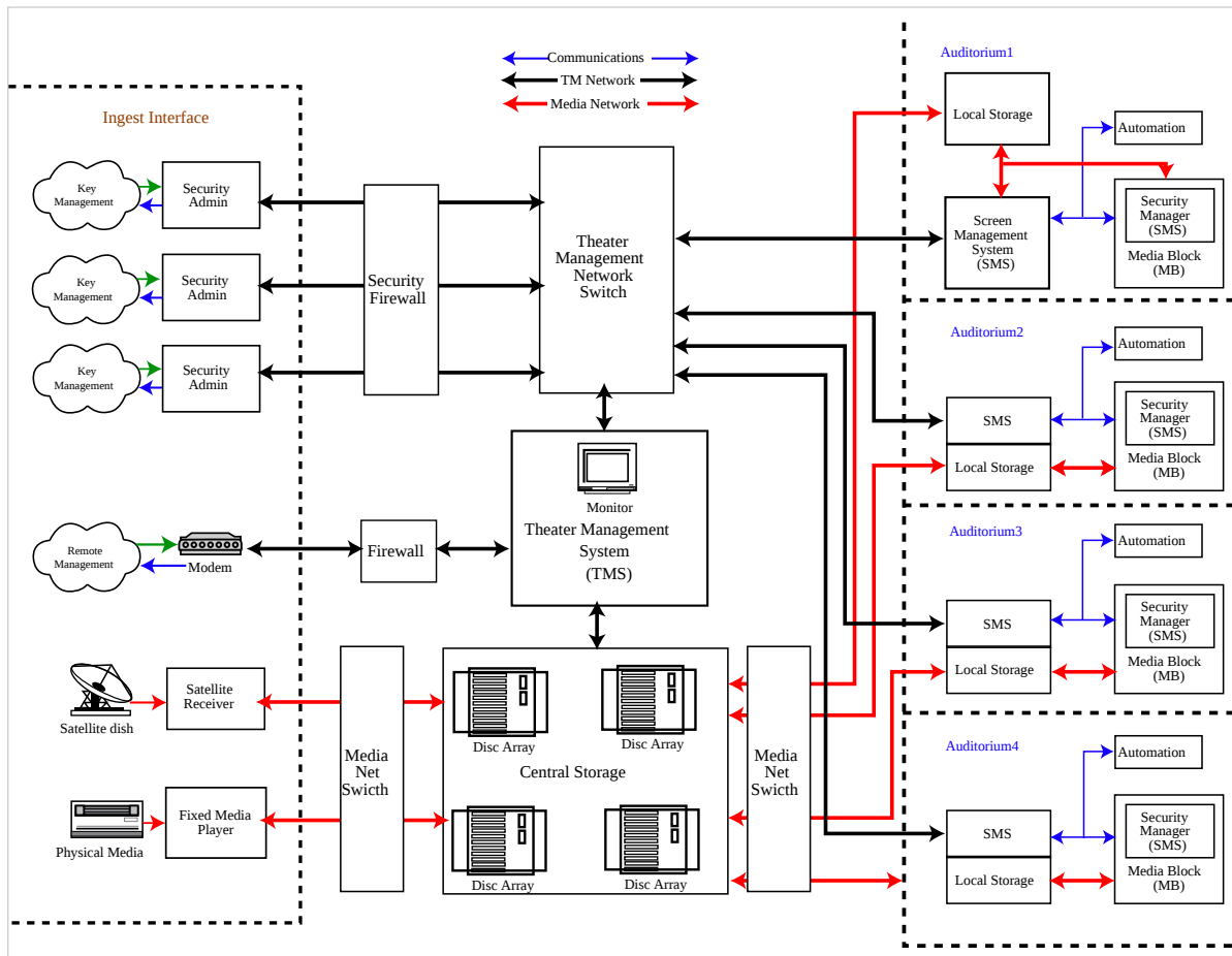
Figure 13: Multiplex Theater System Architecture
