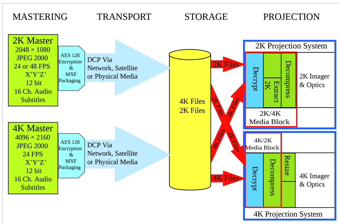
Figure 3: Hierarchical Image Structure
