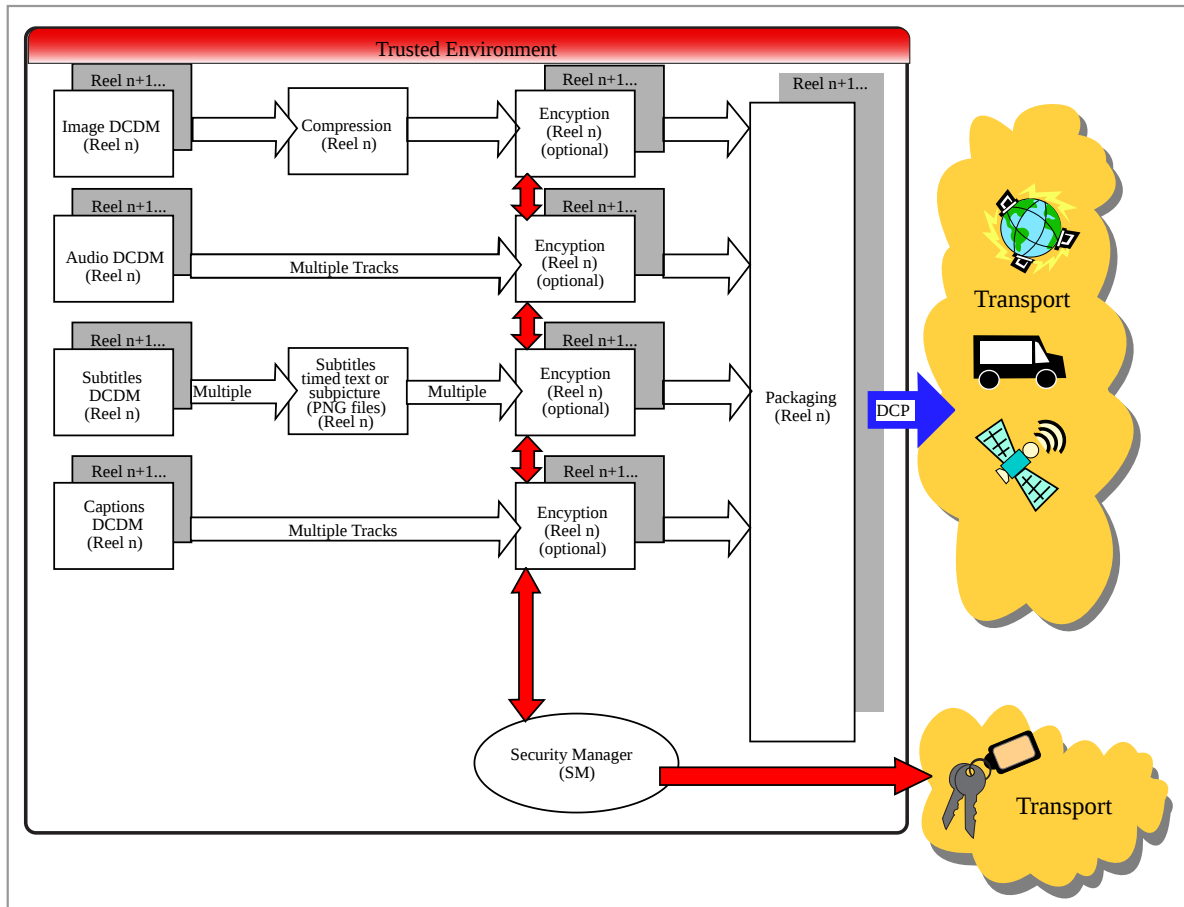
Figure 1: System Overview Functional Encode Flow
