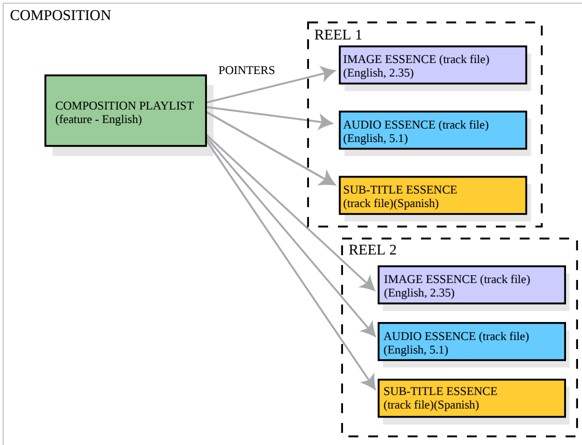
Figure 5: Example Composition Playlist
