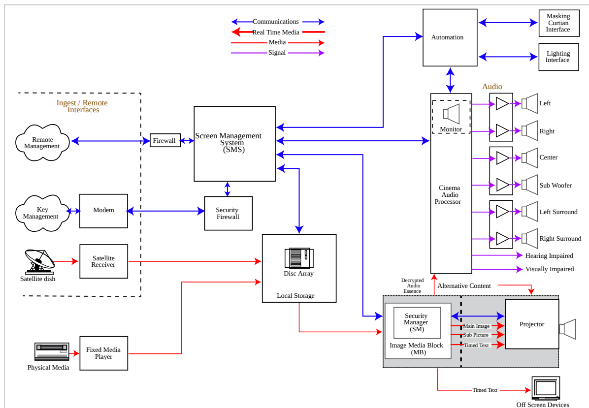
Figure 10: Single-Screen System Architecture
