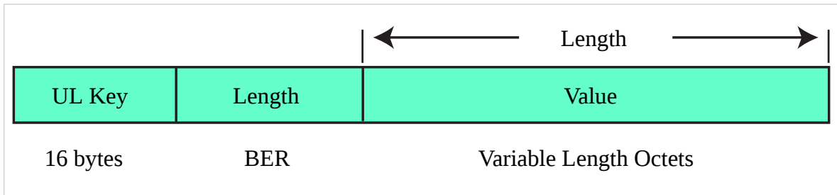
Figure 9: Example of KLV Coding
