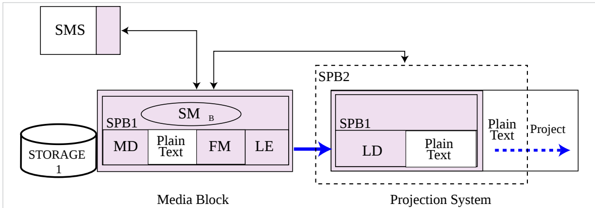
Figure 11: Media Block Server Configuration [4]
