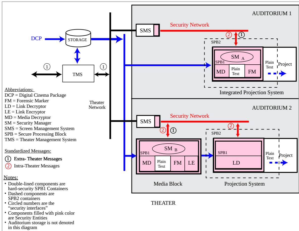
Figure 15: Digital Cinema Auditorium Security Implementation
