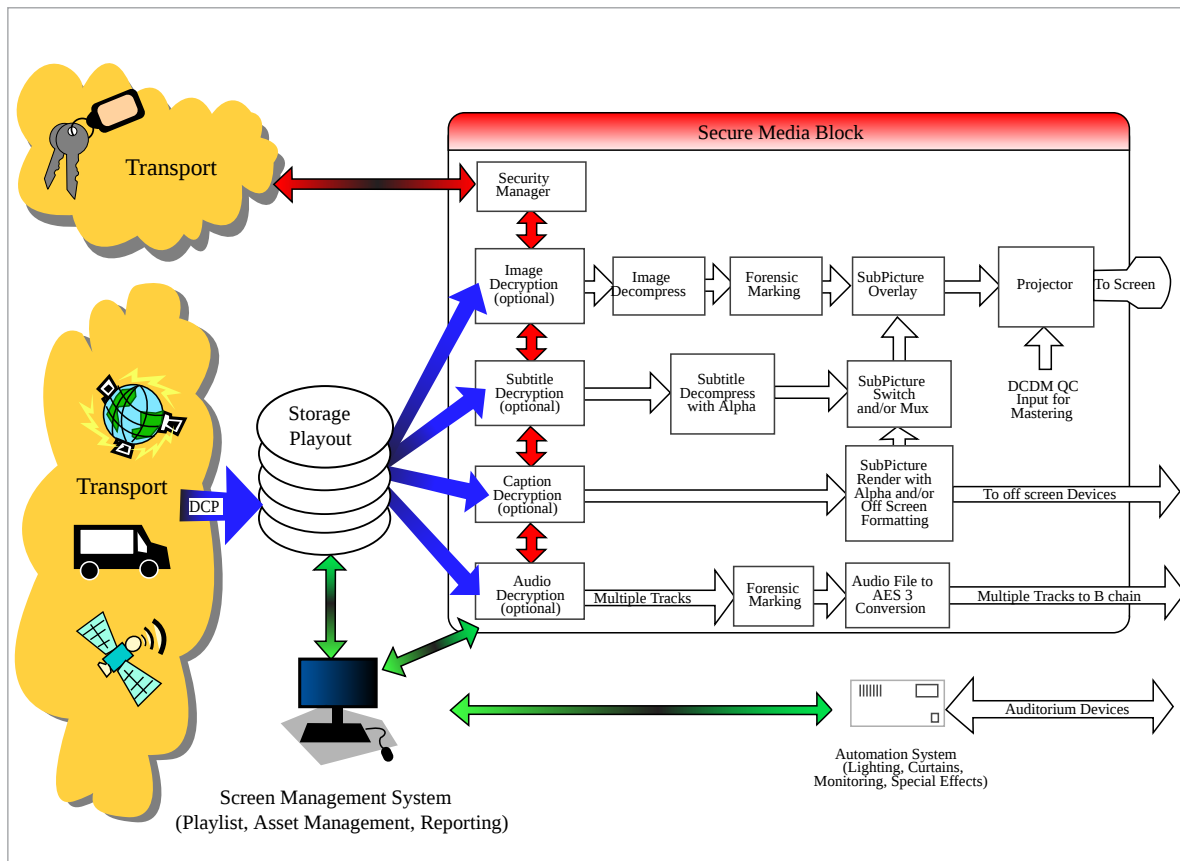
Figure 2: System Overview Functional Decode Flow
