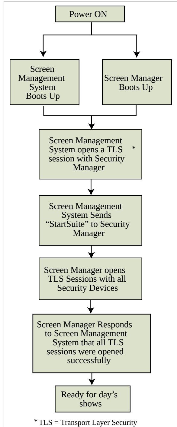
Figure 16: System Start-Up Overview
