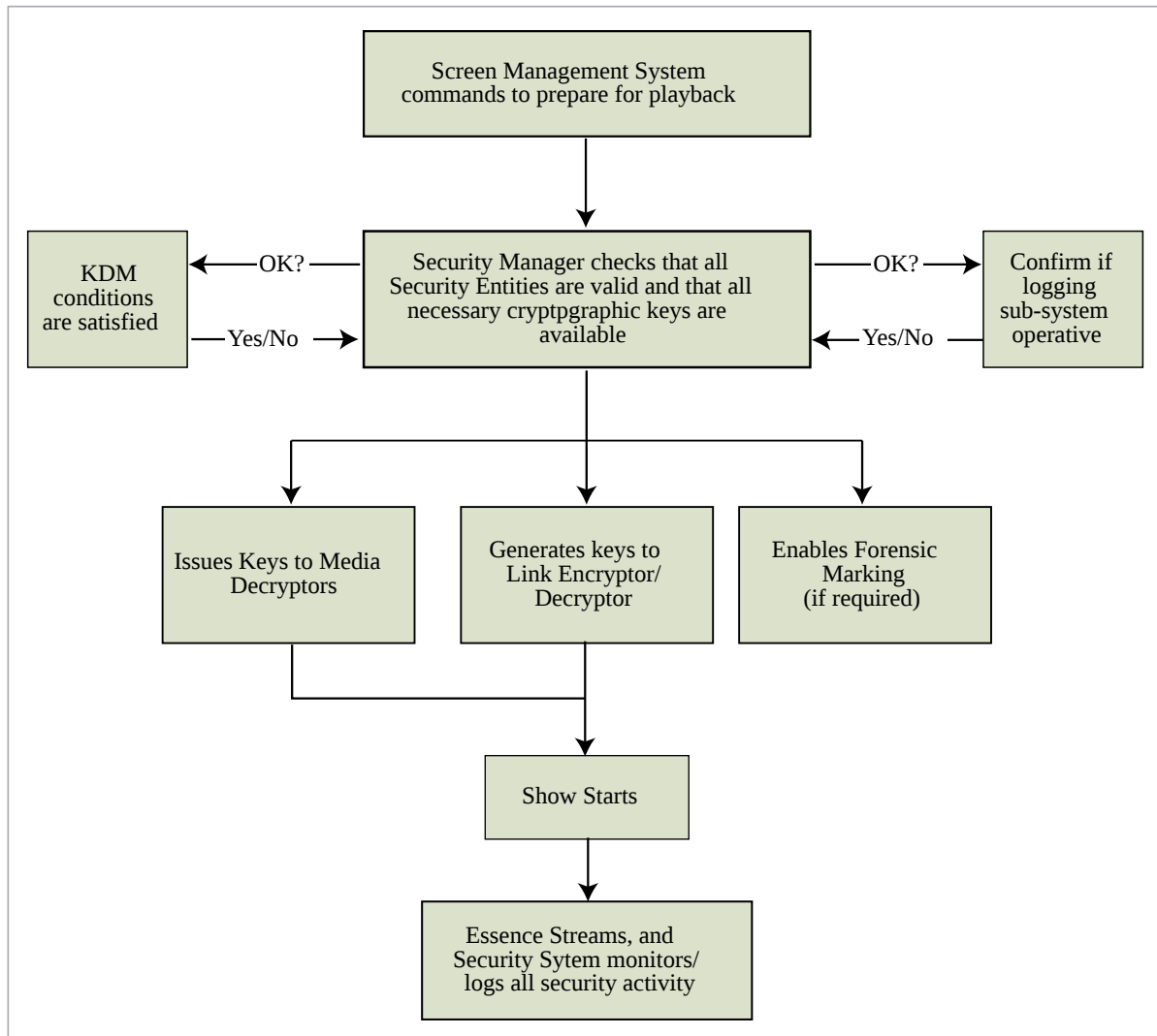
Figure 18: Show Playback Overview
